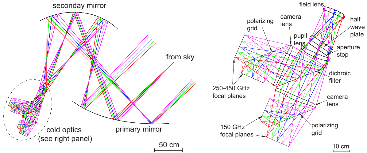
Figure 5. Left panel: The 1.5 m Dragon telescope provides 8 arcminute beams at 150 GHz. Light is coupled from the telescope to the cold optics, seen in close up on the right. Right panel: The cold optics image two perpendicular polarization components from each of the four frequencies onto four focal planes.
