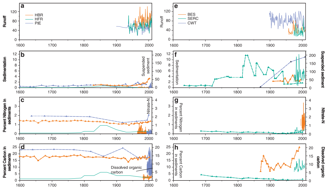
Figure 4. Cross-site comparison of material flux. Panels a and e show the runoff in centimeters per year at each site (data sources: CWT, US Geological Survey [USGS] gauge no. 03513000; SERC, Weller et al. 1986, Jordan et al. 1997, 2003, Correll et al. 1999a, Breitbart et al. 2008; BES, USGS gauge no. 01589300; PIE, USGS gauge no. 01102000; HFR, USGS gauge no. 01174500; HBR, Bailey et al. 2003). Panels b and f show two series where they were available: sedimentation rates in millimeters per year (the dashed lines with triangles) and contemporary suspended sediment concentrations leaving the watershed in milligrams per liter (the solid lines). (Sedimentation rate data sources: CWT, Leigh 2010; SERC, Elliott and Brush 2006; BES, Mason et al. 2004; PIE, Köster et al. 2005; HBR, McLauchlan et al. 2007. Suspended sediment data sources: SERC, Jordan et al. 1997, 2003, Correll et al. 1999b, Gallegos et al. 2005, Breitbart et al. 2008; PIE, http://ecosystems.mbl.edu/pie/data/wat/WAT-VA-Inputs.html ; HFR, estimated as was described in the text). Panels c and g show nitrogen concentrations, both in the sedimentary record (as the percentage nitrogen, the dashed line with triangles) and in surface waters (the level of nitrate-nitrogen in milligrams per liter, the solid line). The SERC data is depicted as the percentage organic nitrogen, not the total nitrogen. (Sedimentary nitrogen data sources: SERC, Elliott and Brush 2006; PIE, Köster et al. 2005; HBR, McLauchlan et al. 2007. Surface water nitrate data sources: SERC, Weller et al. 1986, Jordan et al. 1997, 2003, Correll et al. 1999c, Breitbart et al. 2008; BES, www.beslter.org/frame7-page_1_verbose.html and historic USGS water-quality data for gauge no. 01589300; PIE, http://ecosystems.mbl.edu/pie/data/wat/WAT-VA-Inputs.html ; HFR, estimated as was described in the text; HBR, Jordan et al. 1997, 2003, Hong et al. 2005). Panels d and h show carbon data, both in the sedimentary record (as percentage carbon, the dashed line with triangles) and in surface waters (dissolved organic carbon in milligrams per liter, the solid line). The SERC data is depicted as the percentage organic carbon, not the total carbon, and the BES data are depicted as the percentage of organic matter. (Sedimentary carbon data sources: SERC, Elliott and Brush 2006; BES, Mason et al. 2004; PIE, Köster et al. 2005; HBR, McLauchlan et al. 2007. Dissolved organic carbon data sources: SERC, Jordan et al. 1997, 2003, Correll et al. 2001, Breitbart et al. 2008; PIE, http://ecosystems.mbl.edu/pie/data/wat/WAT-VA-Inputs.html ; HFR, estimated as was described in the text; HBR, Johnson et al. 2000).
